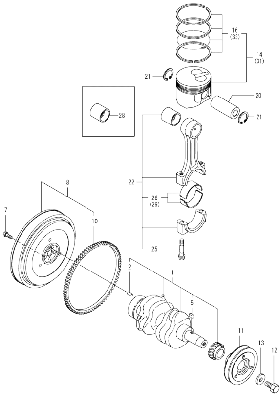
Fig.7. CRANKSHAFT & PISTON
