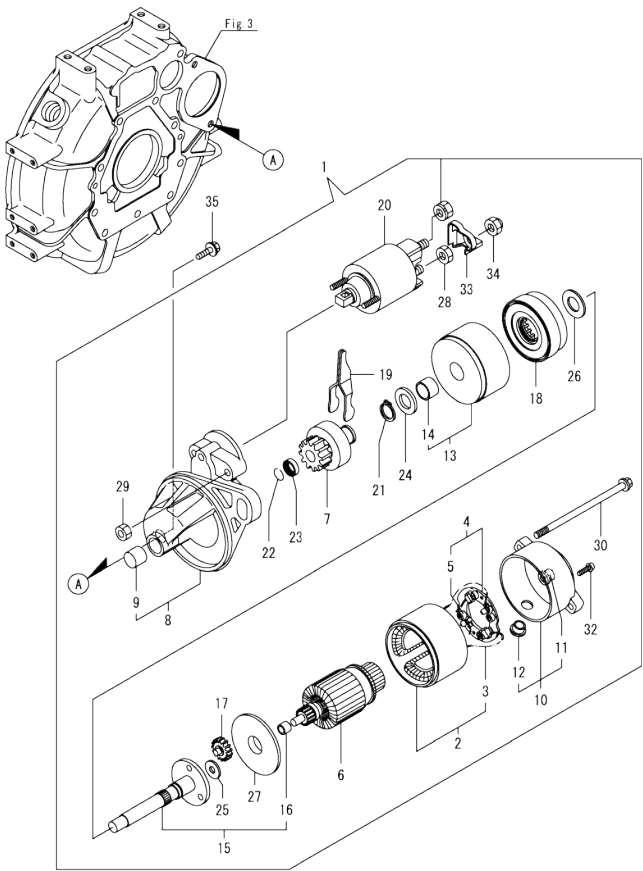
Fig.14. STARTER MOTOR
