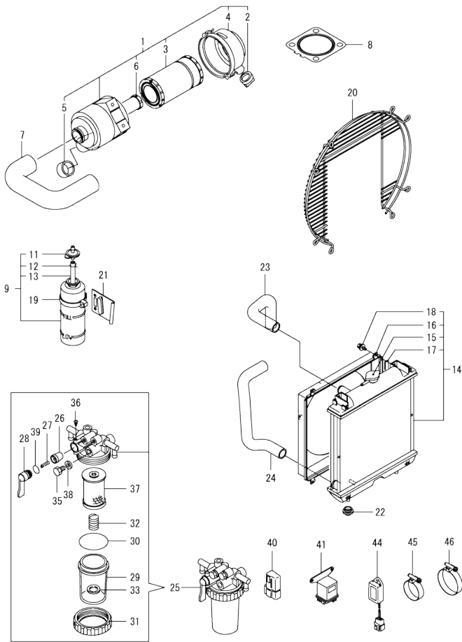
Fig.16. ACCESSORY
