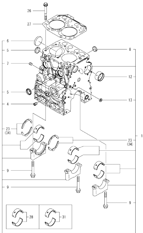
Fig.1. CYLINDER BLOCK
